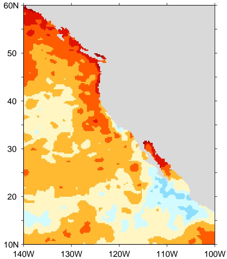
April–May–June 2005 AVHRR SST anomalies (C, wrt 2000–08)
