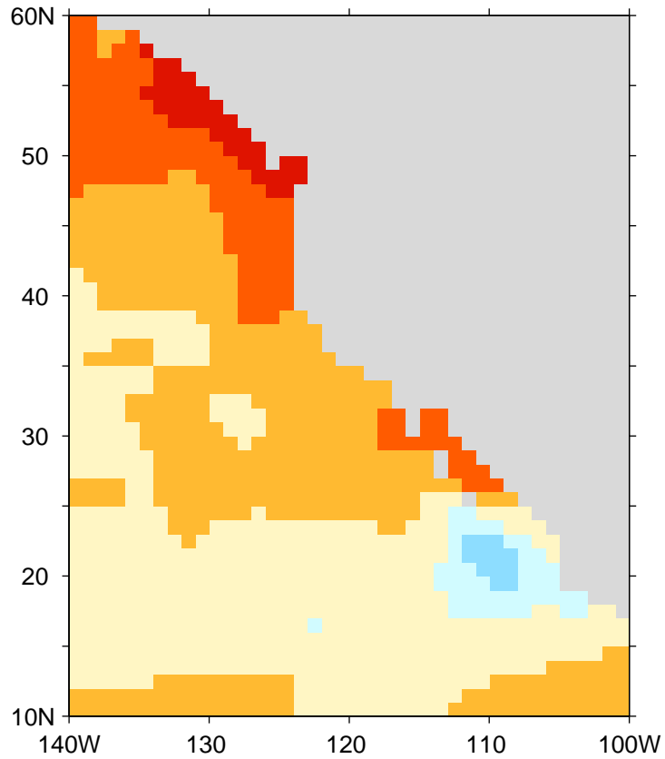
April–May–June 2005 HadISST SST anomalies (C, wrt 2000–08)
