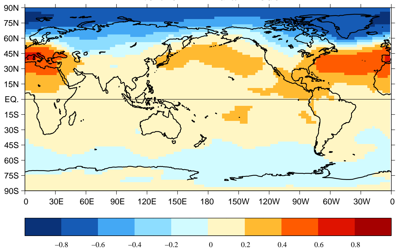
EOF one of NH SLP anomalies for 1948 – March 2010 All calendar months. 18.5% of the variance. Plotted as correlation coefficients.
