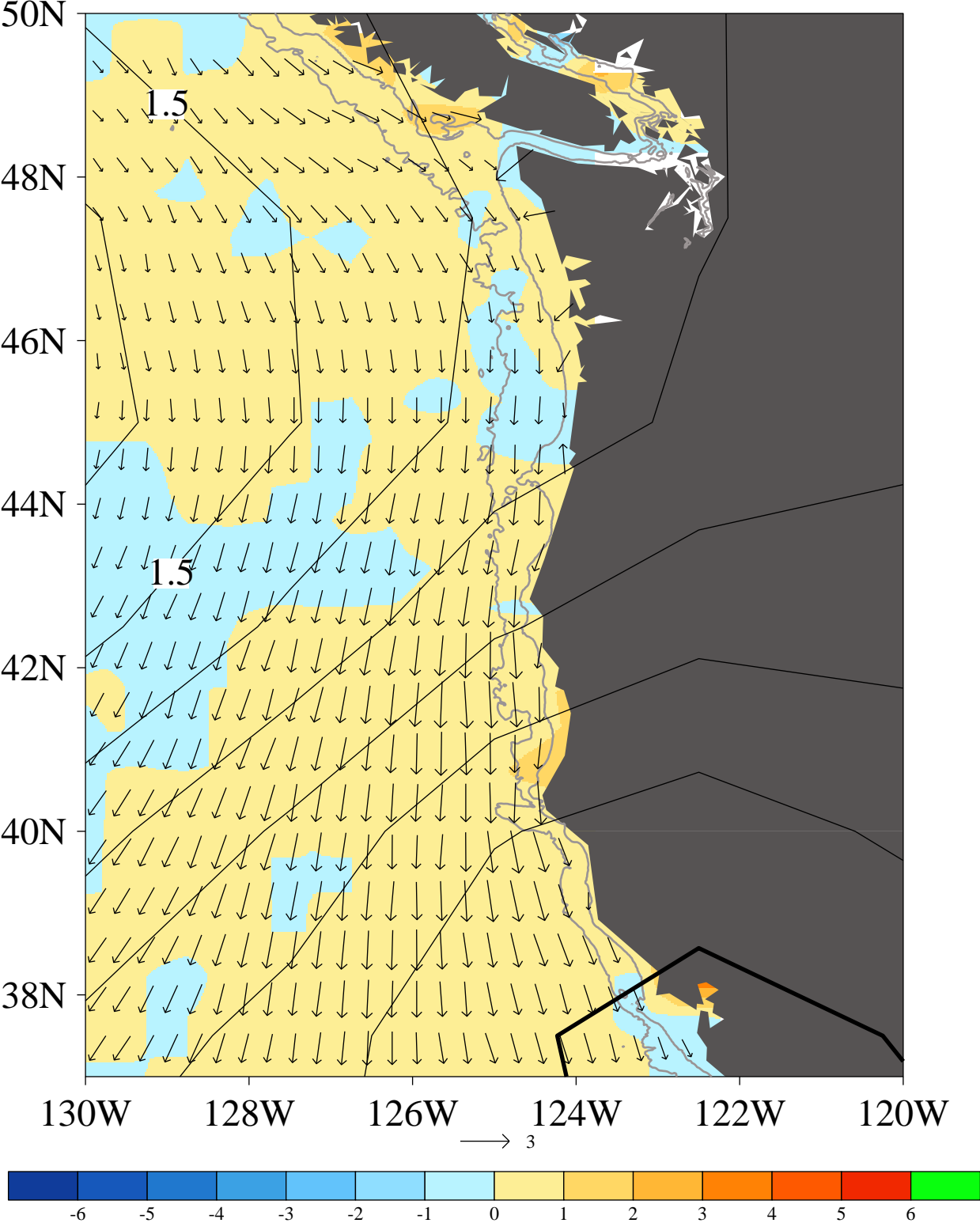
Chlorophyll, wind, and SLP -10 days wrt the Heceta Bank chlorophyll maxima
