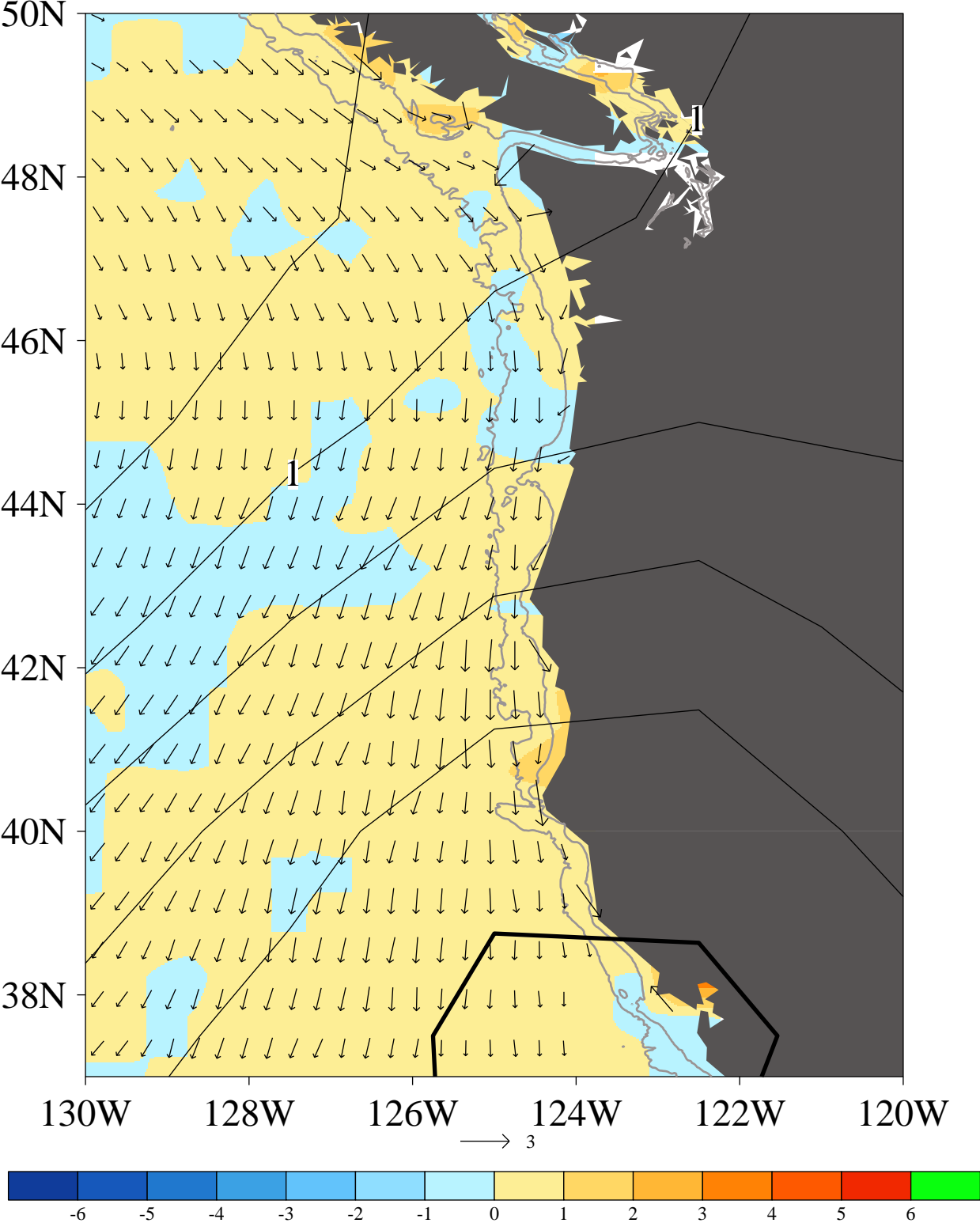
Chlorophyll, wind, and SLP -15 days wrt the Heceta Bank chlorophyll maxima
