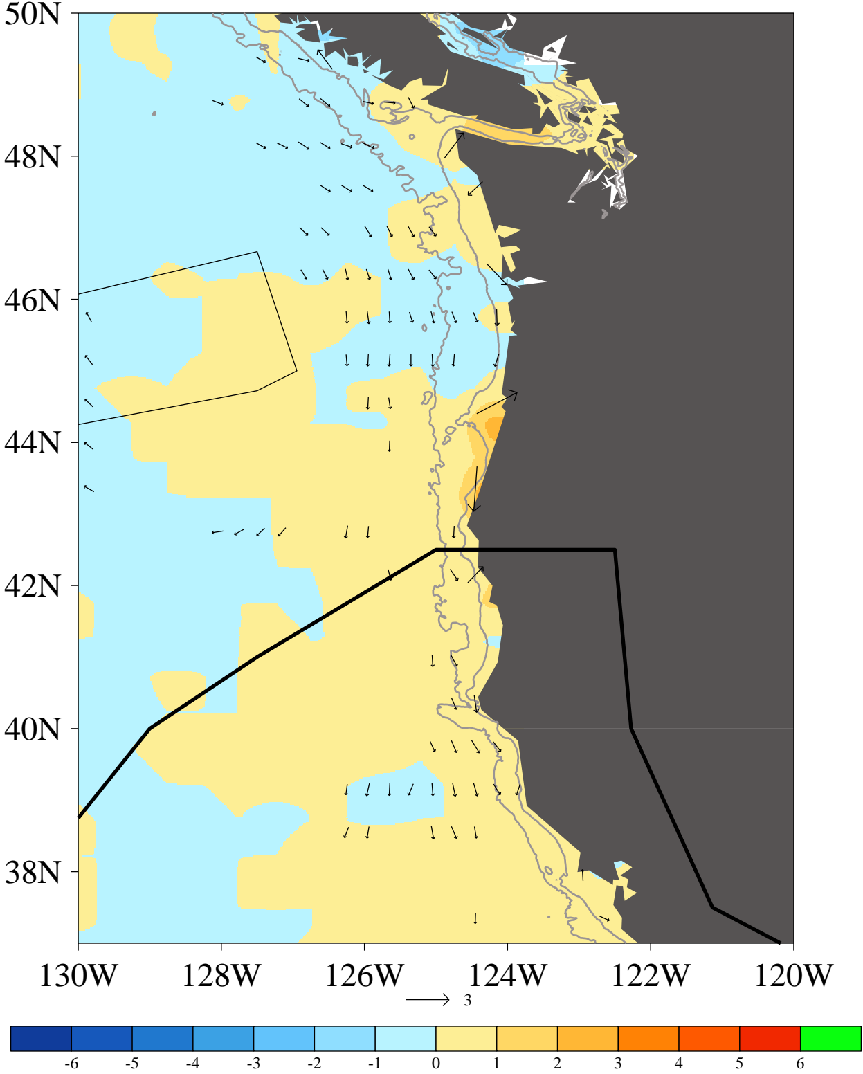
Chlorophyll, wind, and SLP +10 days wrt the S. OR - N. CA chlorophyll maxima
