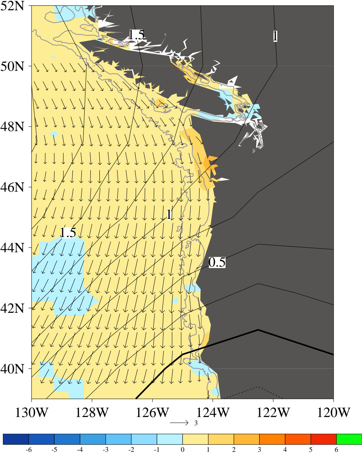
Chlorophyll, wind, and SLP -10 days wrt the S. WA / N. OR chlorophyll maxima
