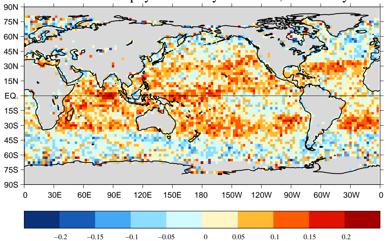
Local corr. chlorophyll–tendency & aerosol, 1998–May2005
