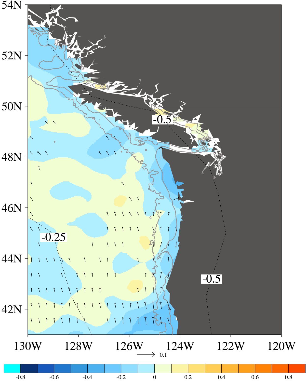
SST, wind stress, and SLP +10 days wrt the Vancouver I. chlorophyll maxima
