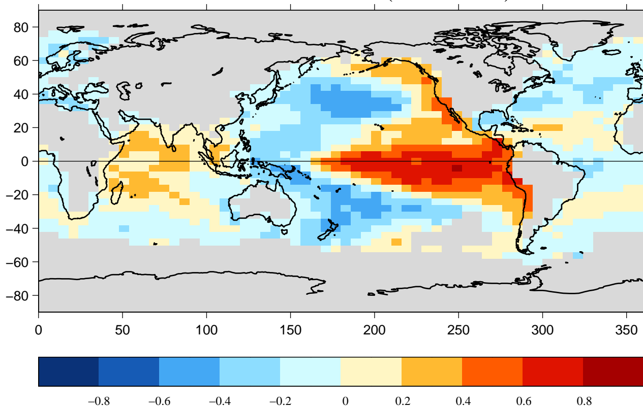
Correlation G & SST (1900–2005)
