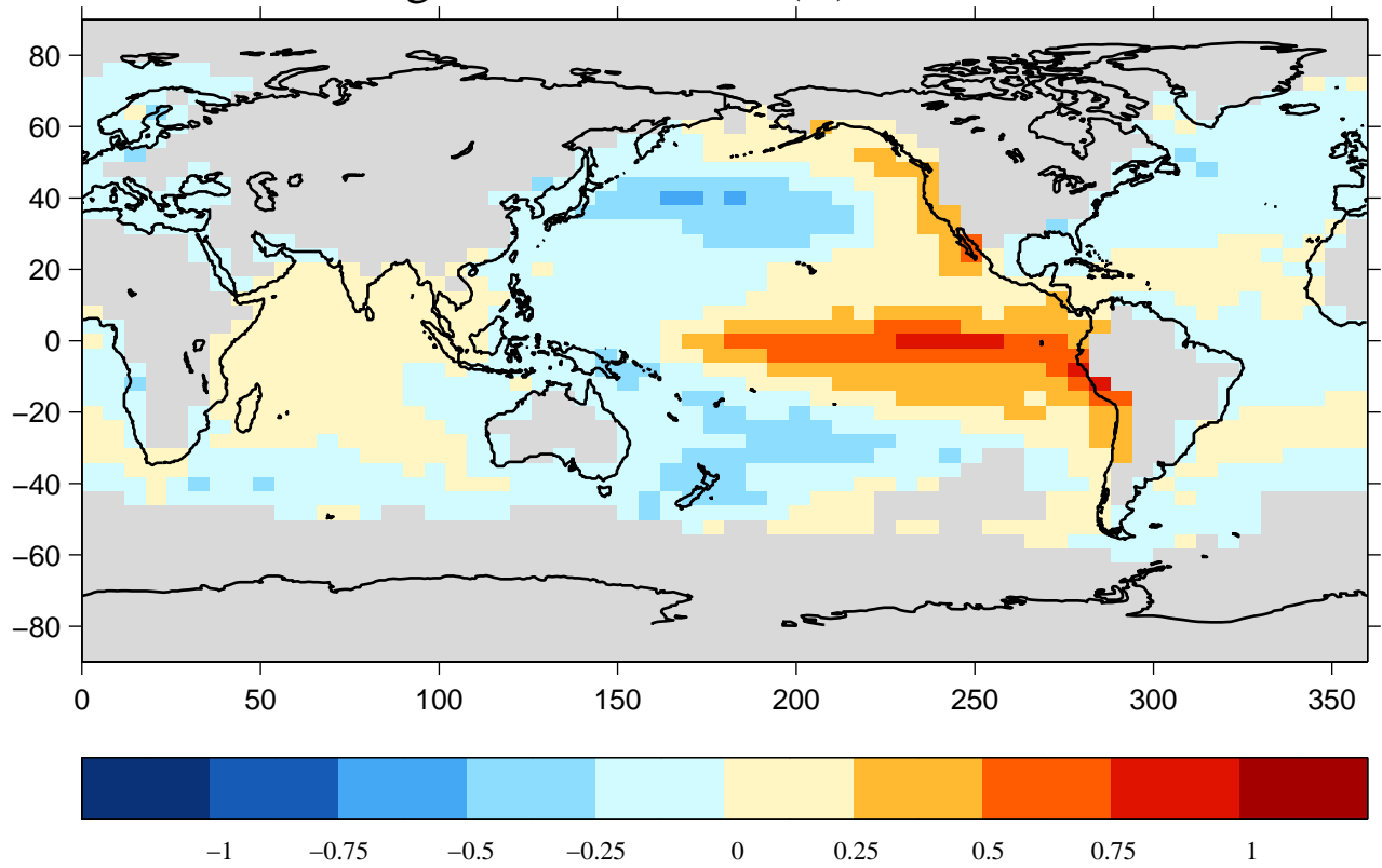
Regress SST onto G (C) 1900–2005
