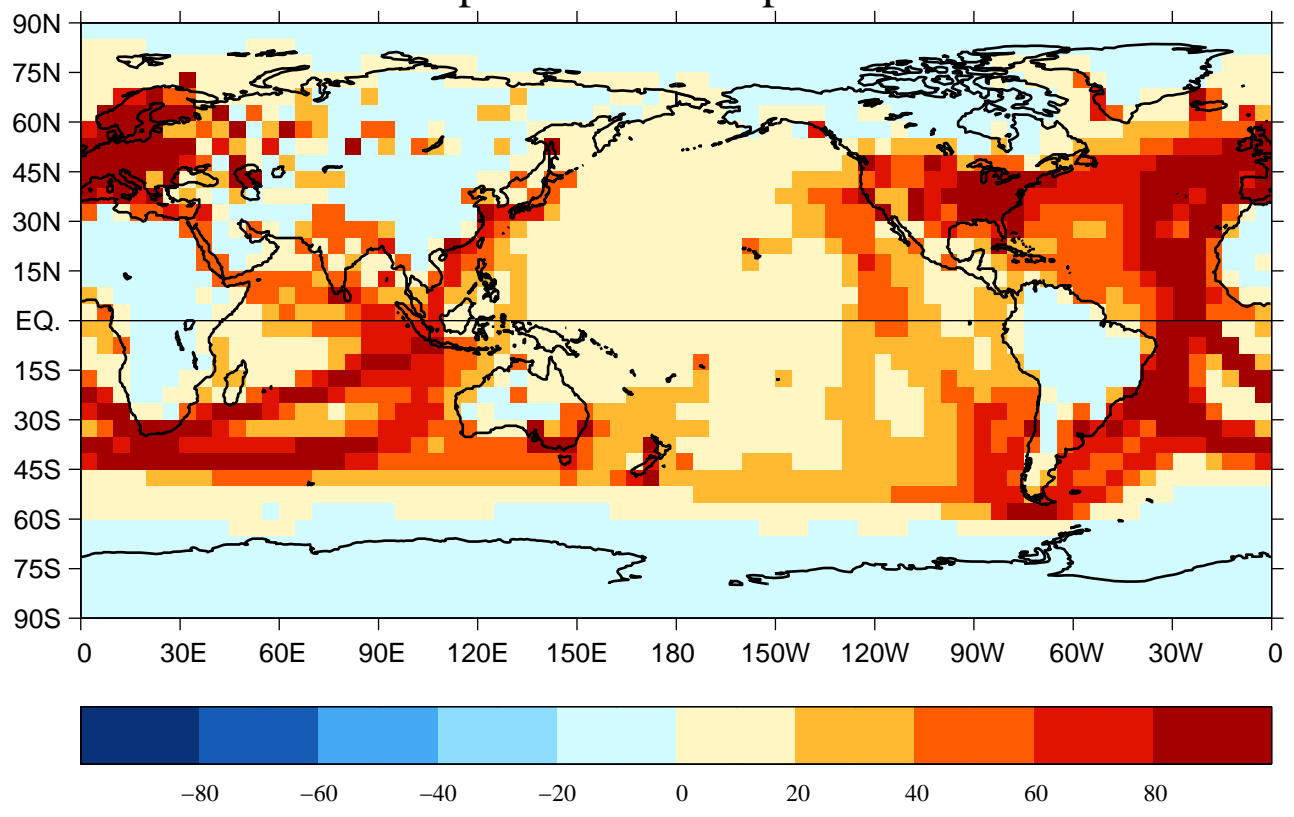
HadCRUT3 sfc. temperature % complete observations 1850–99
