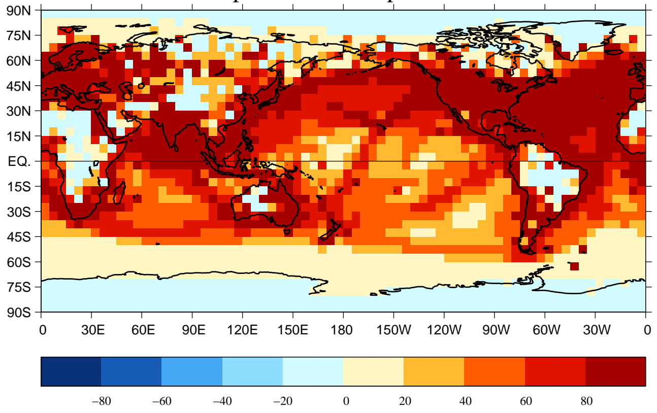
HadCRUT3 sfc. temperature % complete observations 1900–49
