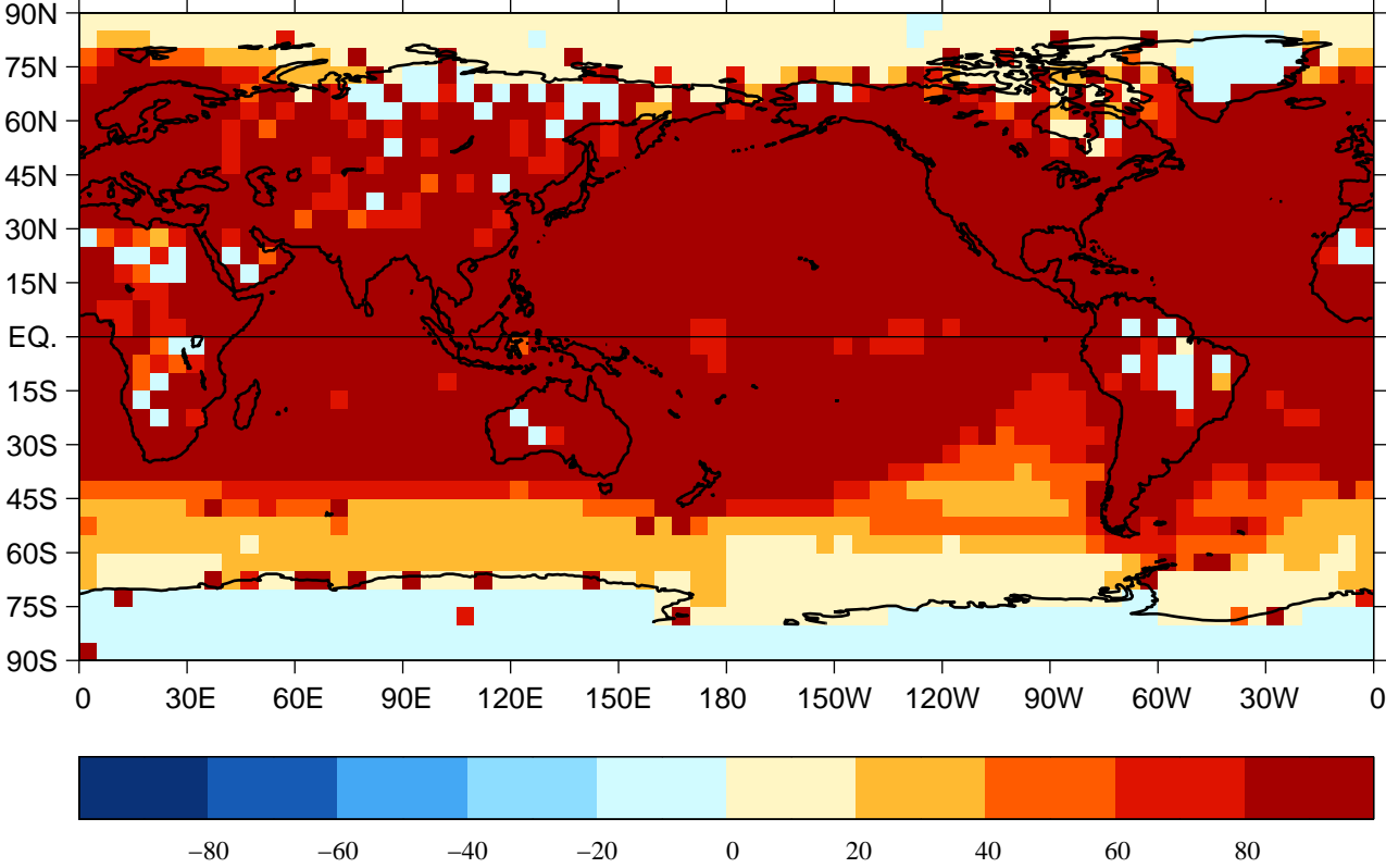
HadCRUT3 sfc. temperature % complete observations 1950–2007
