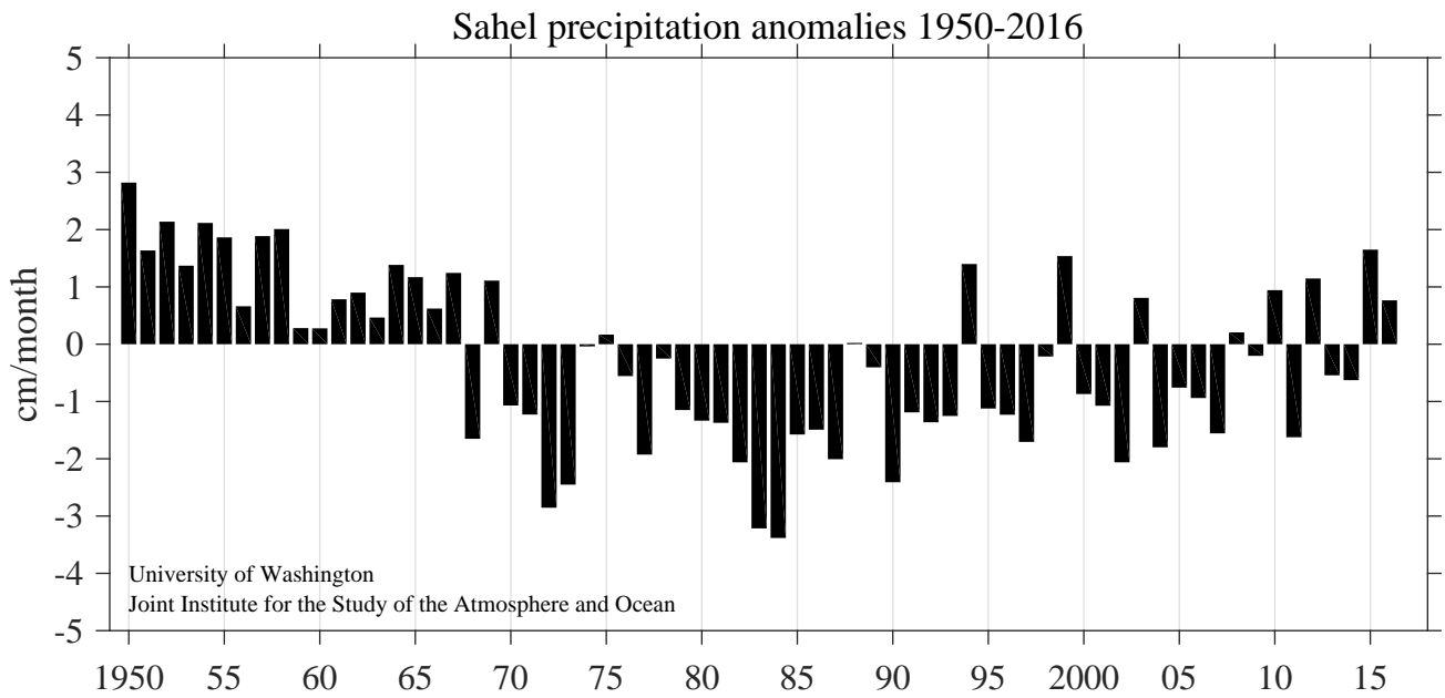
June through October averages over 20-10°N, 20°W-10°E. 1950-2016 climatology Deutscher Wetterdienst Global Precipitation Climatology Centre data
