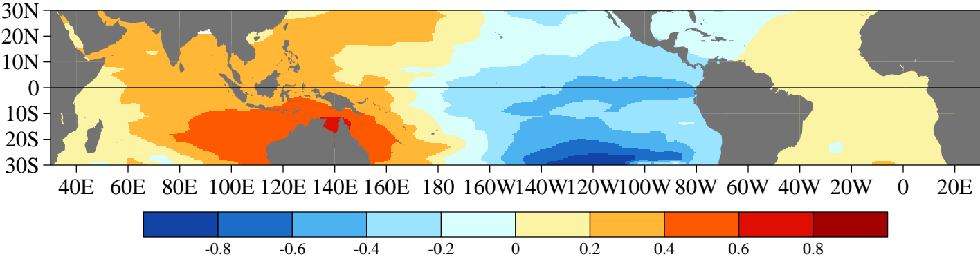
Regression of SLP onto normalized eastern equatorial Pacific SST anomalies (mb), 1950-79
