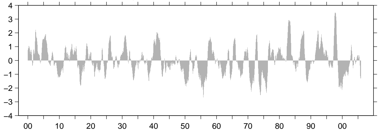
"G" (dimensionless) 1900–2005
