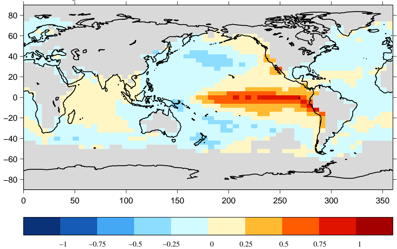
Regress SST onto standardized CTI (C) 1900–2005
