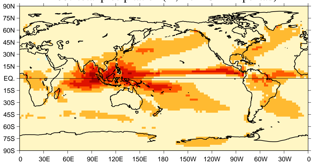
2007 total precipitation (m, from CMAP pentad)
