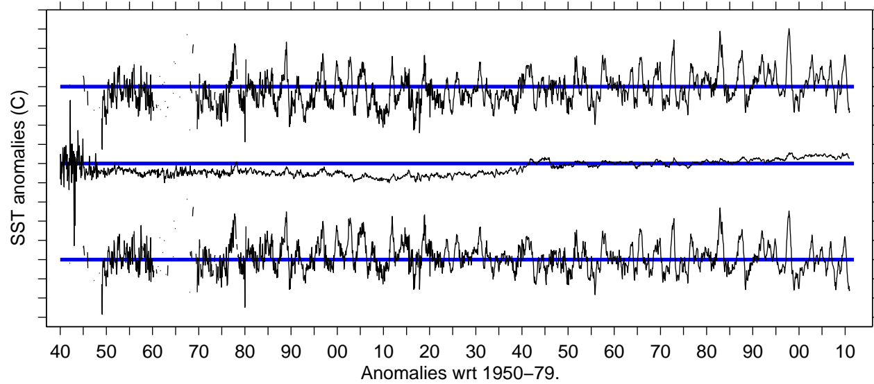
"cti-region", global-mean, "cti" (cti-region minus global mean) 1840- January 2011
