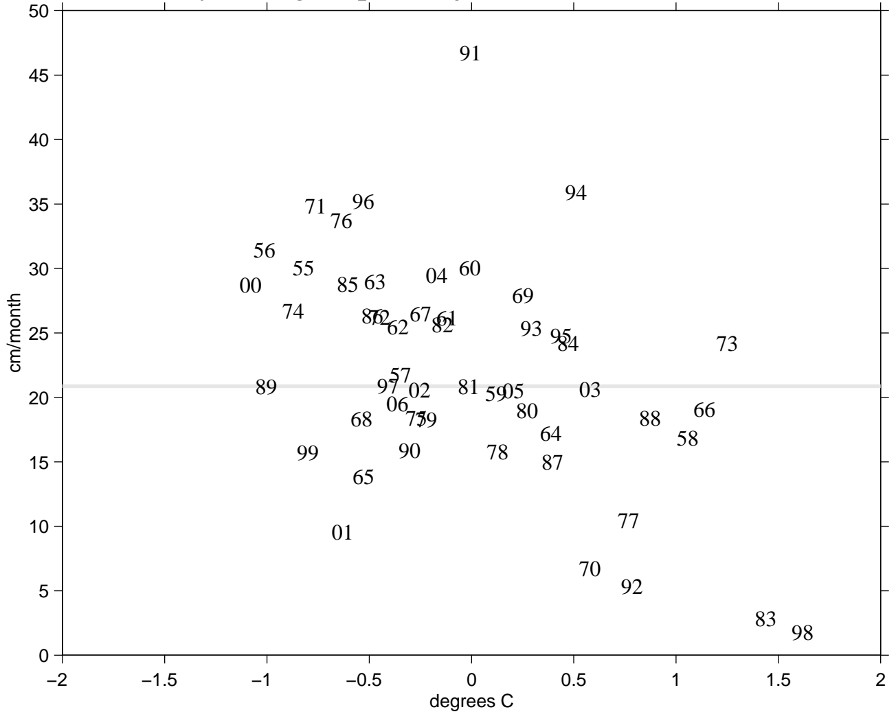
Mean January through April Majuro rainfall versus ENSO SST (C)
