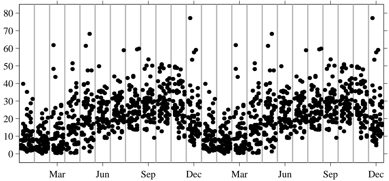
Kwajalein (9N,168E) precipitation (cm) 1946–2006
