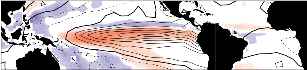
Figure 21. Sea surface temperature anomalies (contour interval 0.2°C) and ocean rainfall anomalies during a typical warm episode of the ENSO cycle. Enhanced rainfall, indicated by the red shading, is observed over the region of above-normal sea surface temperature, and reduced rainfall, indicated by the blue shading, is observed throughout much of the surrounding region and over the tropical Atlantic adjacent to Northeast Brazil.
