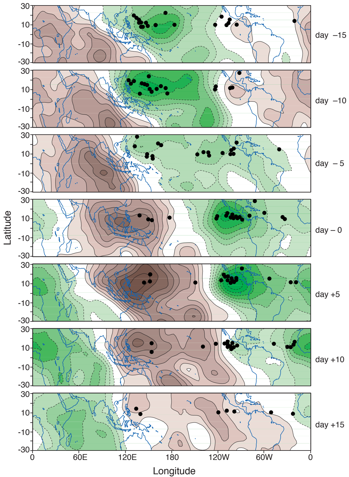
Figure 29. Compositing evolution of 200 hPa velocity potential anomalies ( 10^6 \text{ m}^2 \text{ s}^{-1} ) and points of origin of weather systems that developed into hurricanes or typhoons ( \bullet ).
