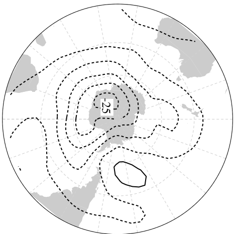
Regression on SH annular mode
