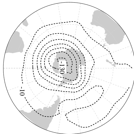
Trends per 15-years
