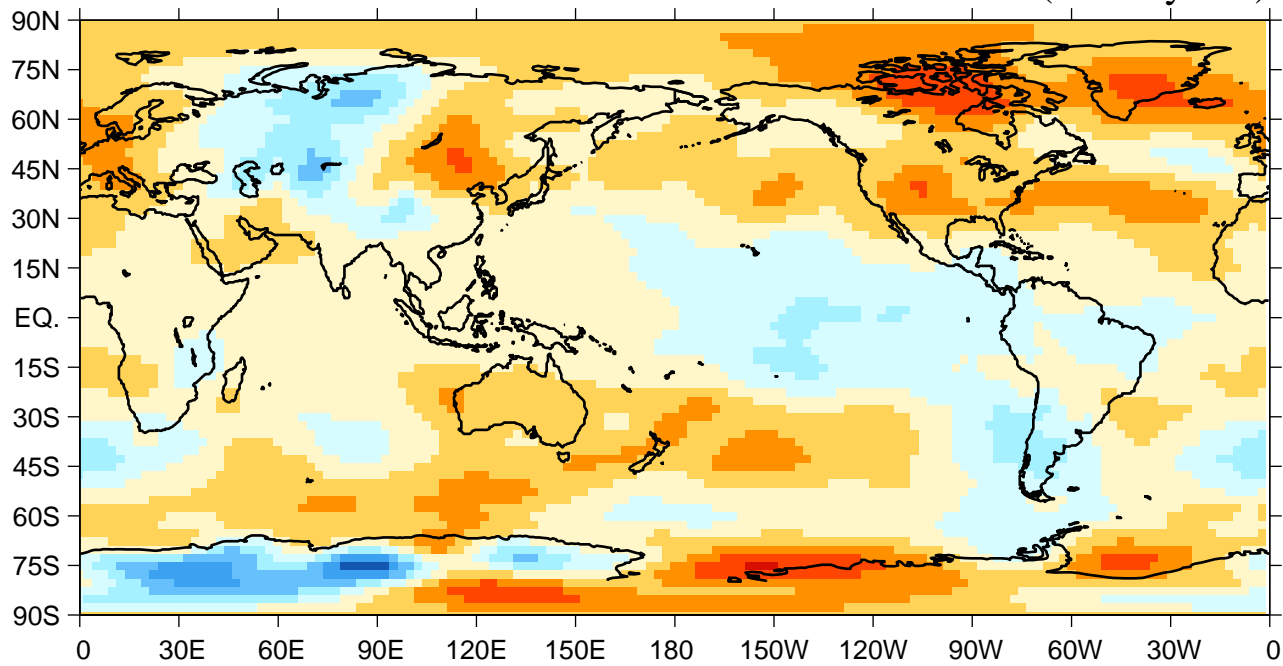
Annual mean 300–850mbZ thickness trend 1979–2003 (m/25–years)
